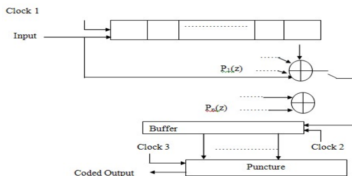
Figure 3.8: Generation of Convolutional Code
