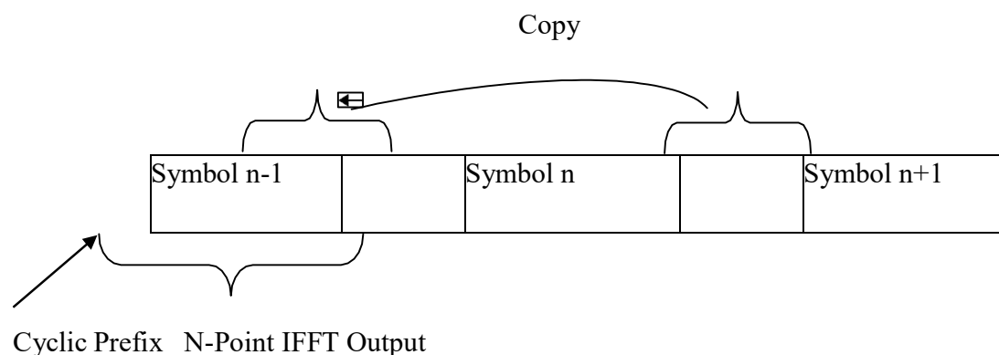
Figure 3.3: OFDM Signal with Cyclic Prefix
