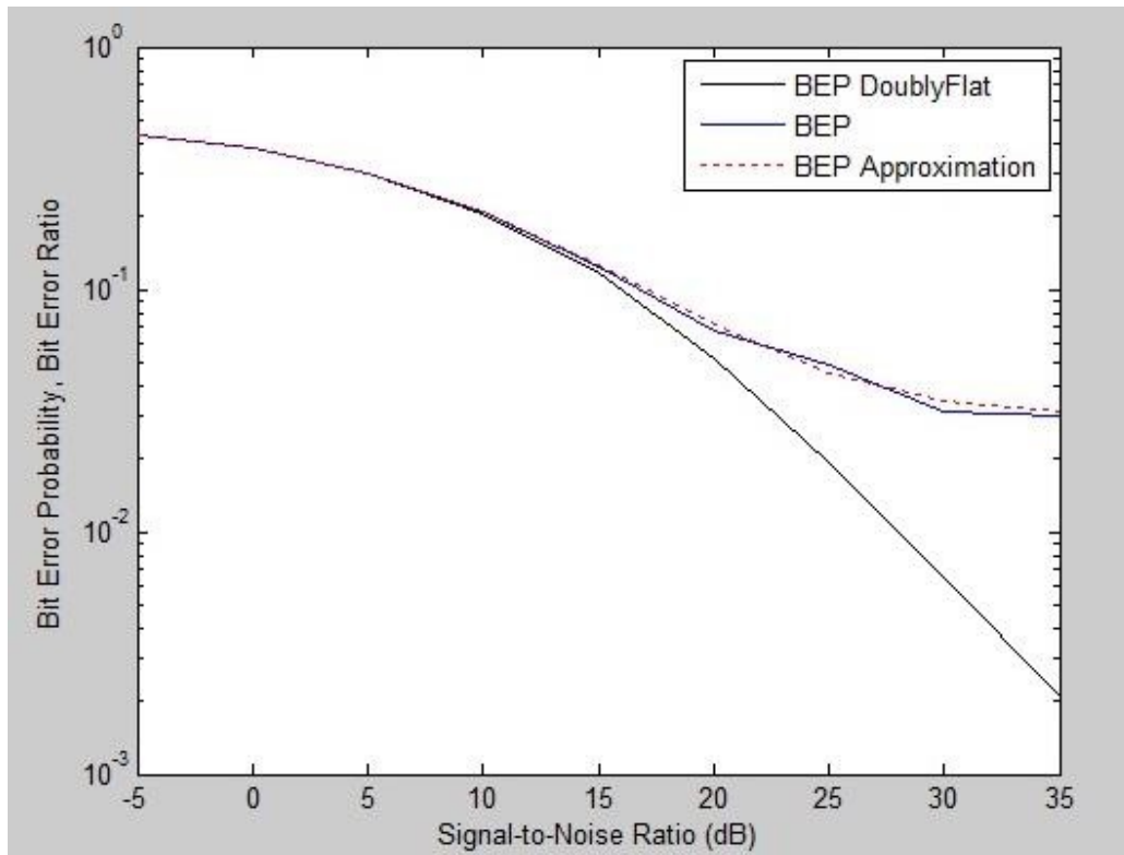
Figure 4.3: SNR vs BEP
