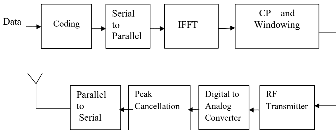
Figure 3.4: OFDM Transmitter with Peak Cancellation Data
