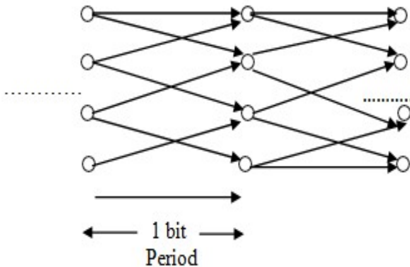
Figure 3.9: State Diagram of Convolutional Code
