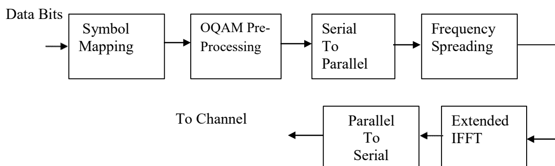
Figure 3.17:FBMC Transmitter
