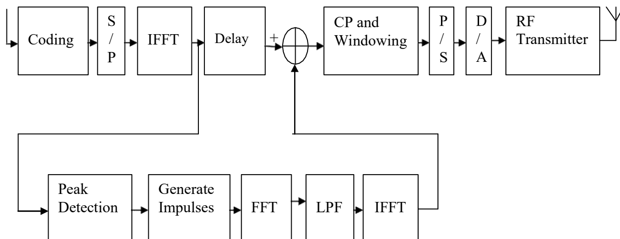
Figure 3.5: Peak cancellation using FFT/IFFT to generate cancellation signal
