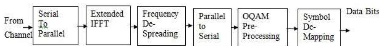
Figure 3.18: FBMC Receiver
