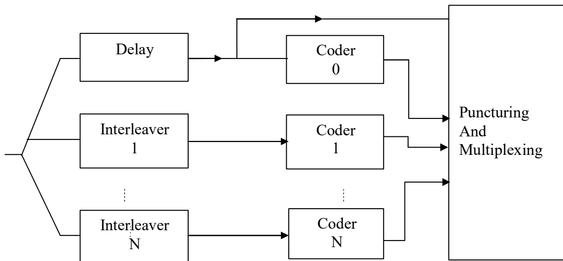
Figure 3.14: A typical turbo encoder
