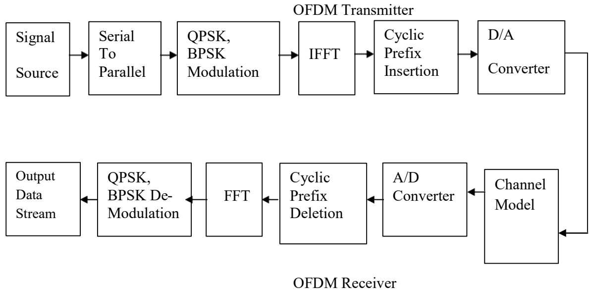
Figure 3.1: OFDM Transmitter and Receiver
