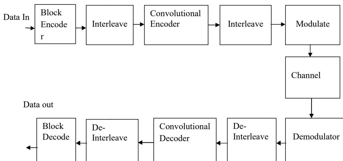
Figure 3.10: Concatenated Coding with Interleaving
