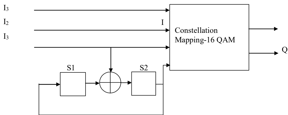
Figure 3.12: Implementation of a Trellis code
