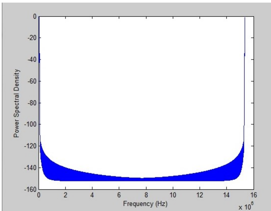
Figure 4.2: Power spectral density
