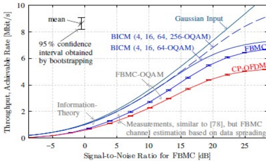
Figure 4.5: Throughput vs SNR
