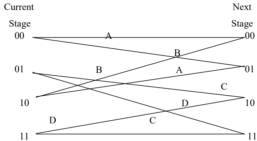
Figure 3.13: State diagram of the Trellis code
