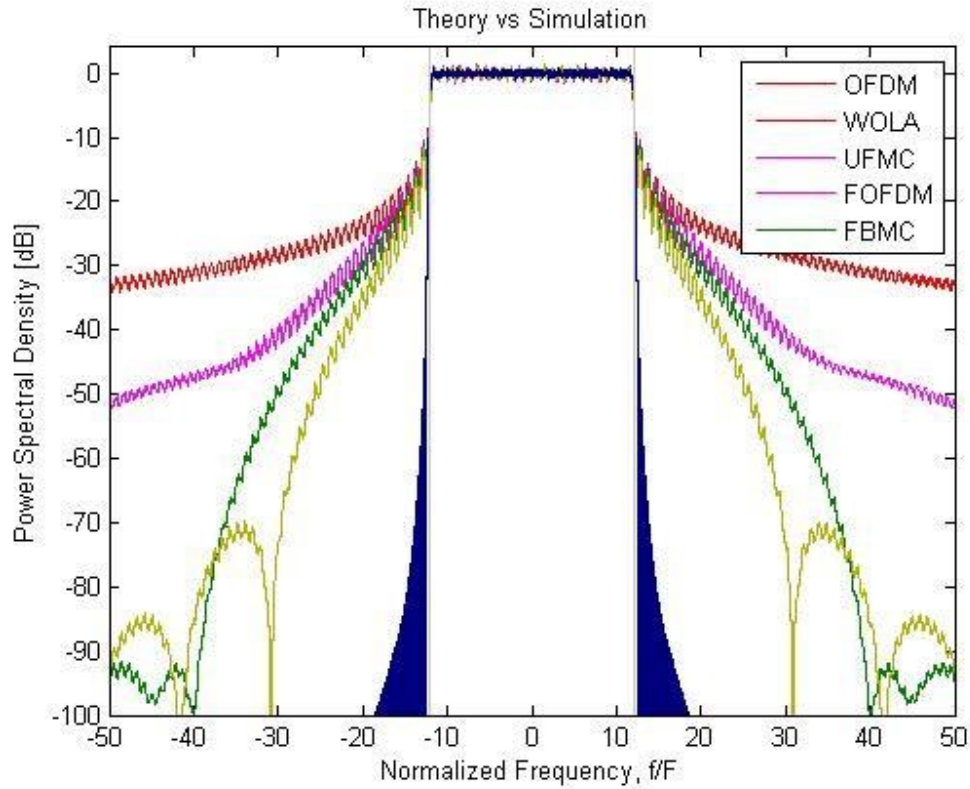
Figure 4.4: FBMC has much better spectral properties compared to CP-OFDM
