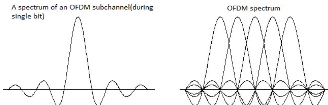
Figure 3.2 : OFDM Spectrum
