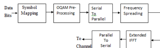
Fig.2 FBMC Transmitter
