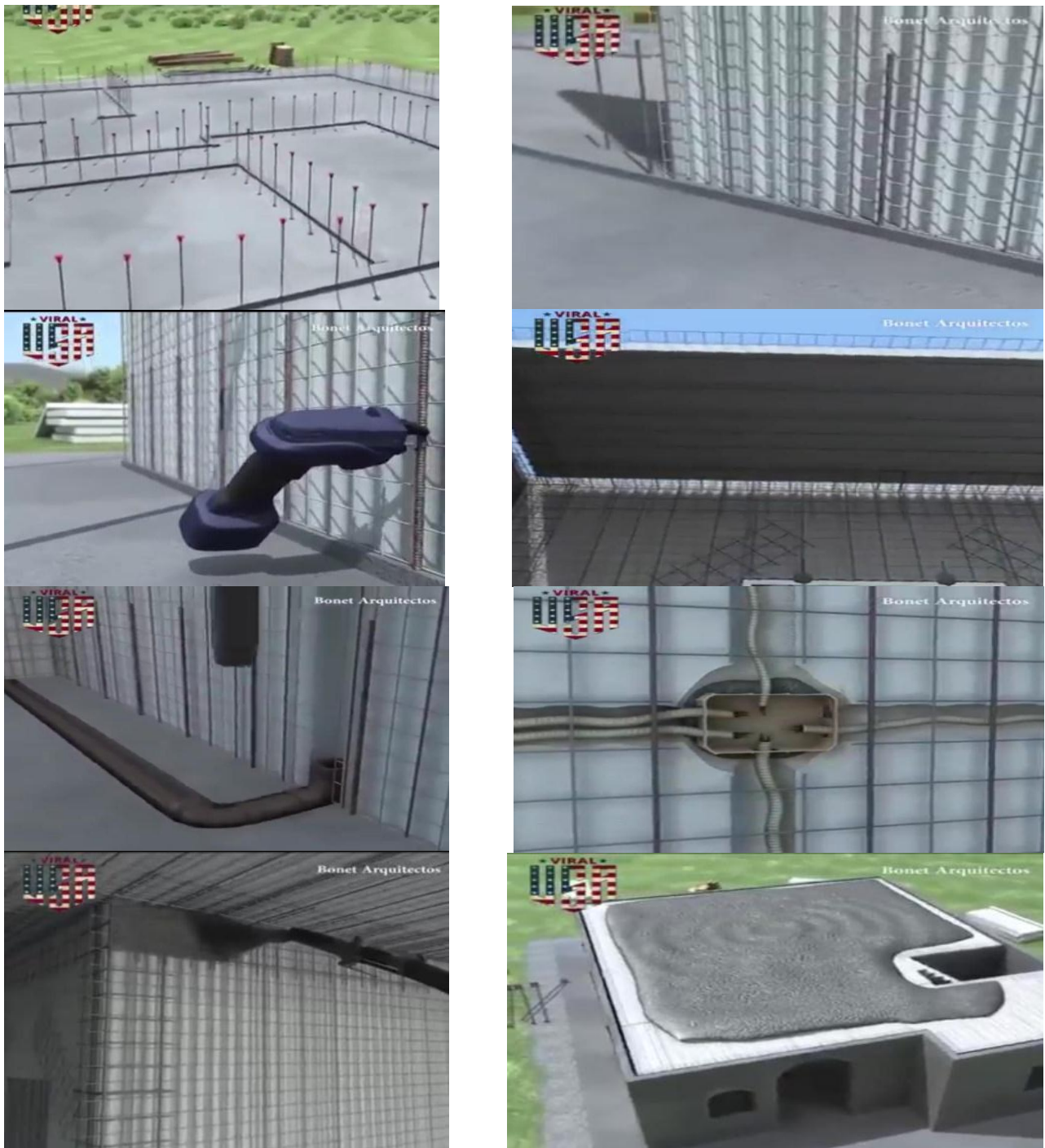
Figure 1.2 Images Showing Installation Procedure of assemblies in EPS core panel building
