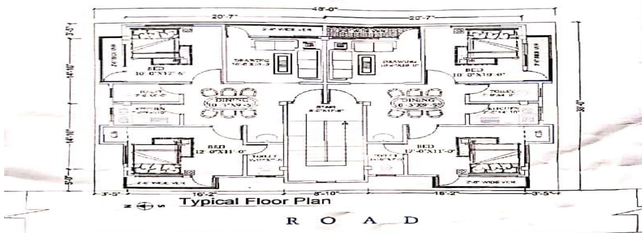
Figure 4.1 Image representing floor plan of the reference building
