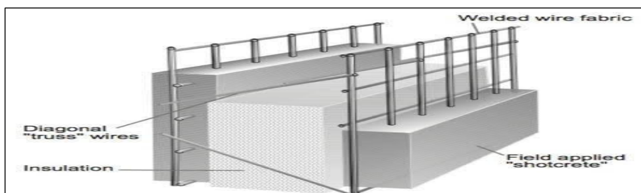
Figure 1.1 Cross-sectional view of EPS core panel
